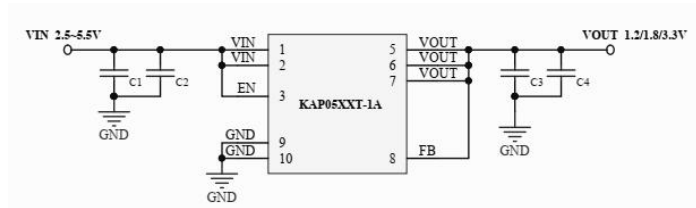
Fig. 2 Typical application circuit
