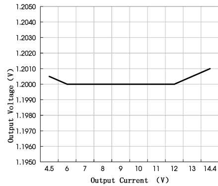
Linear adjustment deviation
