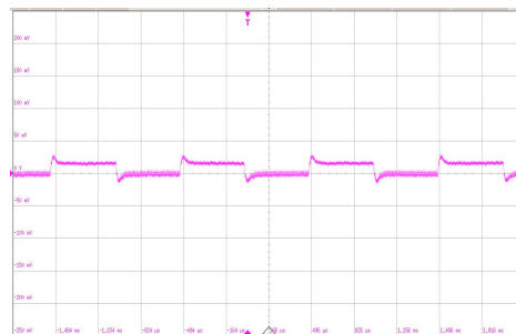
Output Transient Response (50mV/div), 2A/us, 10A-30A-10A, Bandwidth: 20MHz
