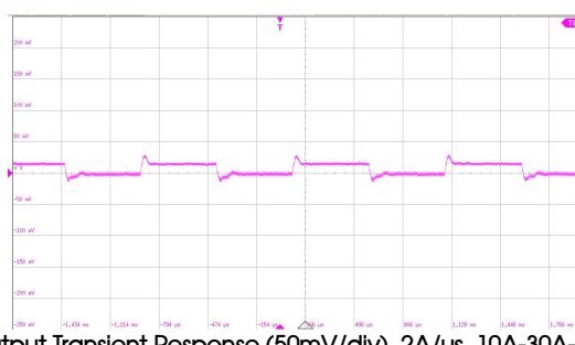
Output Transient Response (50mV/div), 2A/us, 10A-30A-10A, Bandwidth: 20MHz
