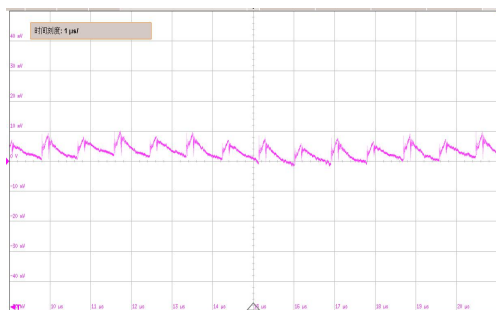
Output ripple & noise(10mV/div), Bandwidth: 20MHz
