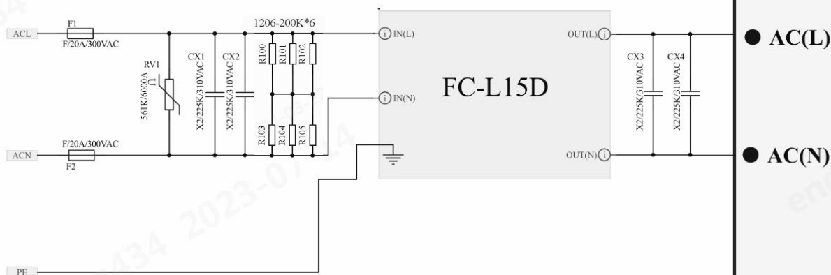
Recommended External Circuit 3
