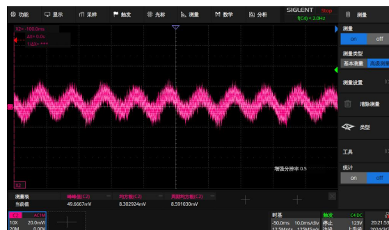
V_{in}=230\text{VAC} full load ripple noise (50mV)/ripple RMS value (8.6mV)
