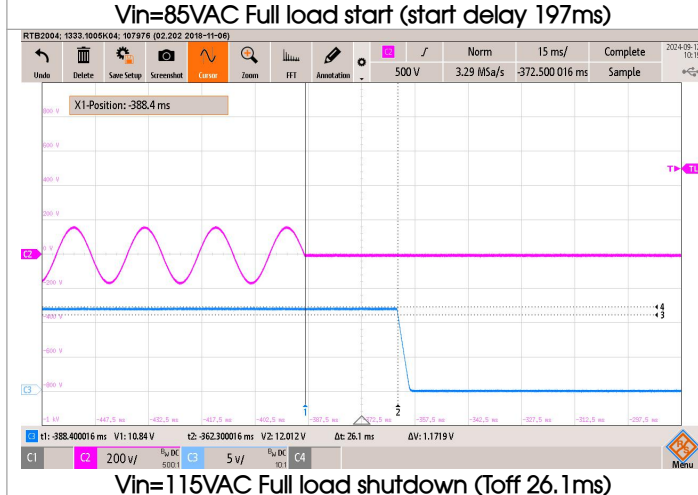
CH2: Input voltage, CH3: Output voltage
