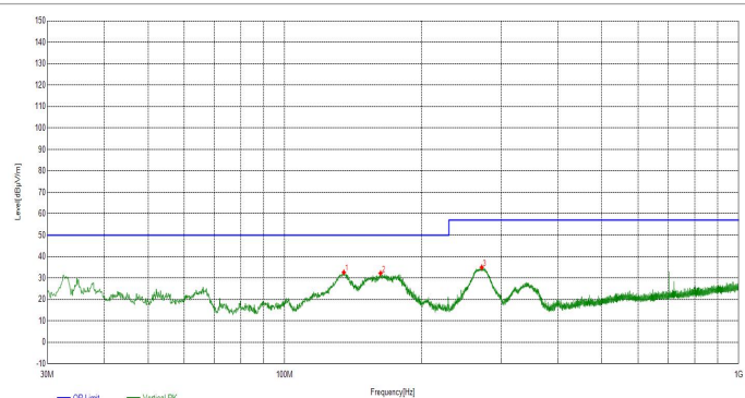
Vertical waveform
