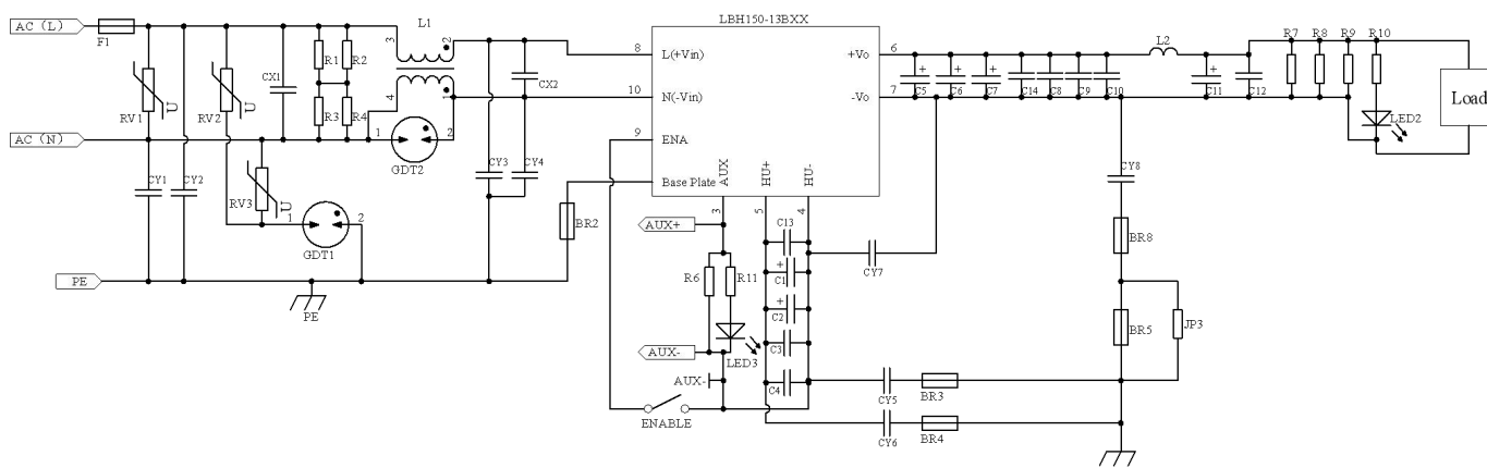
Fig. 1: Recommended circuit 1
