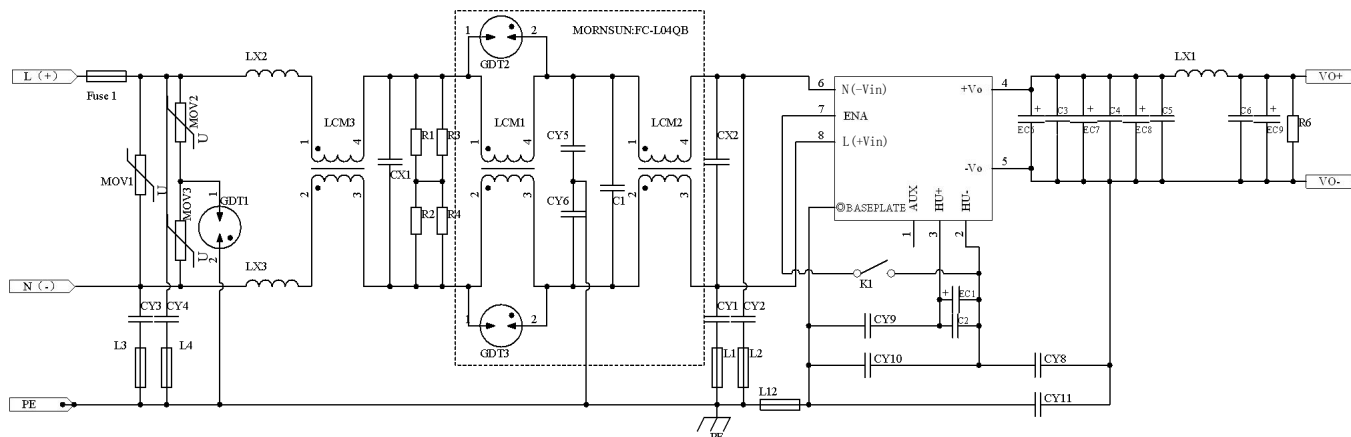
Fig. 2: Recommended circuit 2
