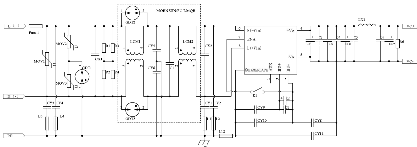
Fig. 1: Recommended circuit 1
