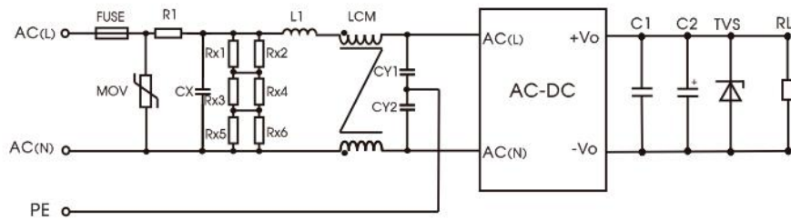
Fig. 2: EMC application circuit with higher requirements (Class I )
