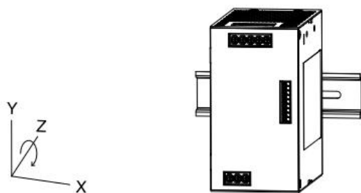
Rotate the installation position (0° Z-Axis)
