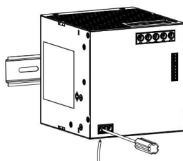
⑤ Turn the Phillips screwdriver to the left to loosen the terminal screws, insert the head of the wire into the bottom of the terminal, and then turn the screwdriver to the right to tighten the terminal screws
