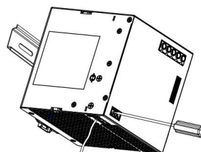
⑥ Turn the Phillips screwdriver to the left to loosen the terminal screw and pull the wire out of the bottom of the terminal
