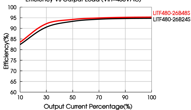
Efficiency Vs Output Load (Vin=400VAC)
