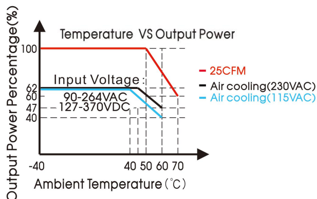
LOF450-20B12/15/18/19 (full load 400W with 25CFM)
