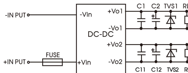
Fig. 1: Typical application circuit
