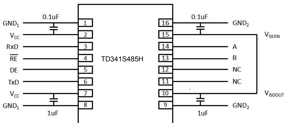
Figure 10. Typical Application of PCB layout
