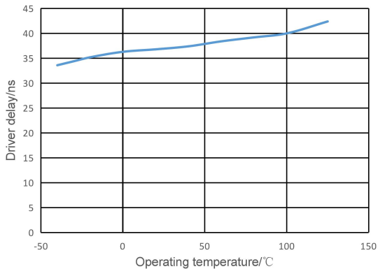
Figure 1. Driver delay vs. Operating Temperature
