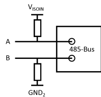
Figure 12. Pull up and drop down resistance connect
