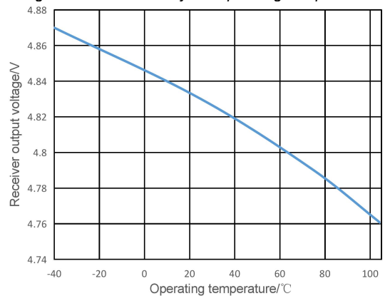
Figure 4. Receiver output high voltage vs. Operating Temperature
