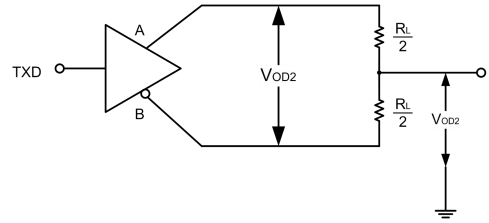
Figure 6. Driver test circuit
