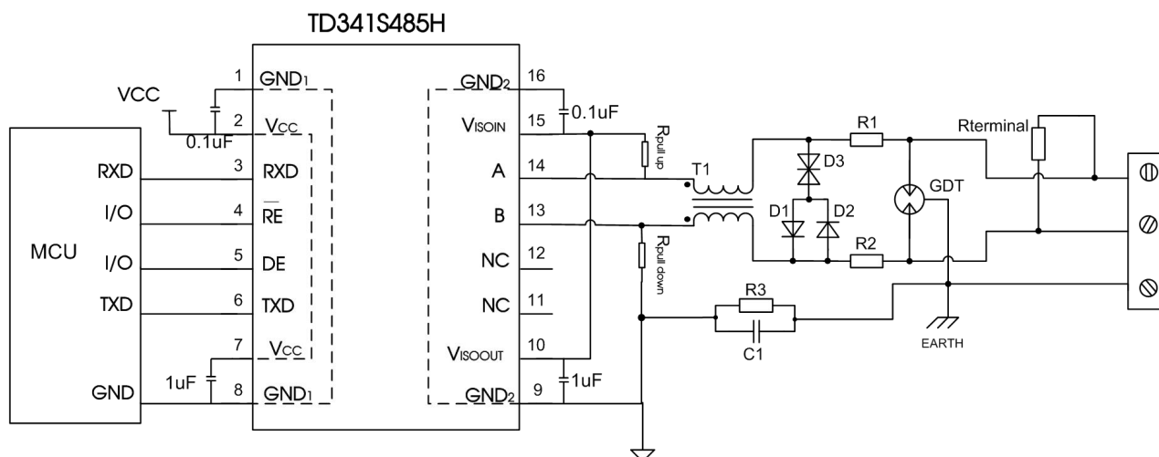
Figure 11. Port protection circuit for harsh environments
