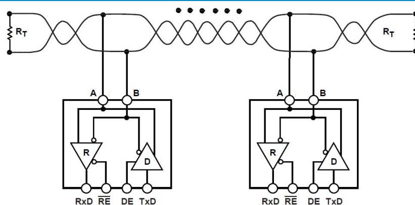
Figure 9. Typical Application Circuit (Half-Duplex Network Topology)
