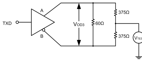
Figure 5. Driver test circuit, VOD with differential mode loading
