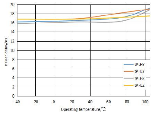
Figure 2. Driver delay vs. Operating temperature
