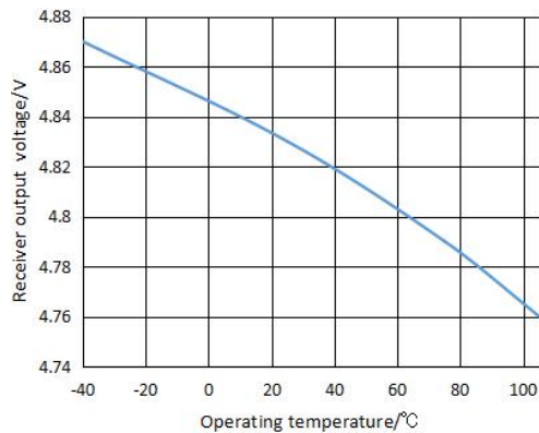
Figure 5. Receiver output high voltage vs. Operating temperature
