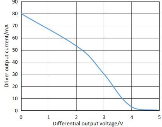
Figure 4. Driver output current vs. Differential output voltage
