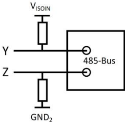
Fig 13. Typical connection of pull-up and pull-down resistors
