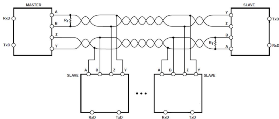
Fig 10. Typical Application Circuit (Full-Duplex Network Topology)
