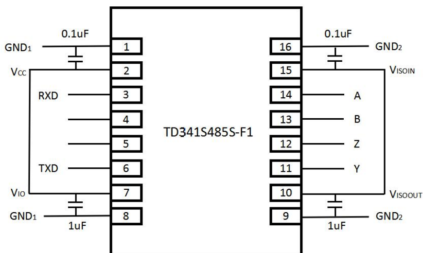
Fig 11. Typical Application of PCB layout
