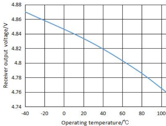
Figure 5. Receiver output high voltage vs. Operating Temperature
