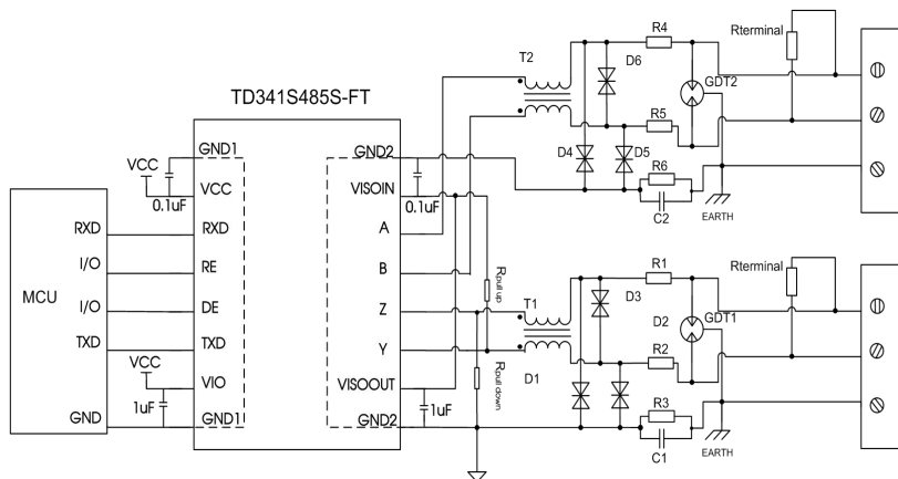
Figure13. Port protection circuit for harsh environments
