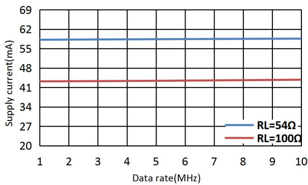
Figure 1. Supply current vs. Data rate
