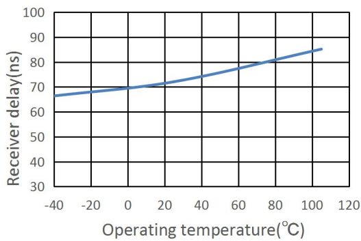
Figure 3. Receiver delay vs. Operating Temperature
