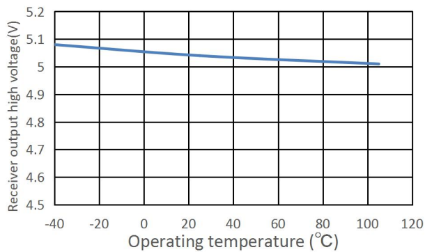
Figure 5. Receiver output high voltage vs. Operating Temperature
