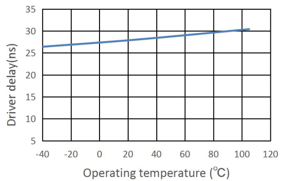
Figure 2. Driver delay vs. Operating Temperature
