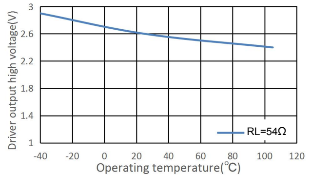
Figure 4. Driver output high voltage vs. Operating Temperature
