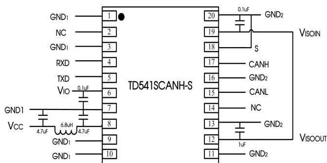
Figure15. EMI Recommended circuit
