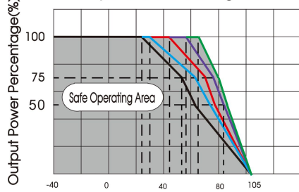
URF1D12QB-100WR3 temperature derating curve (Vin=110V)
