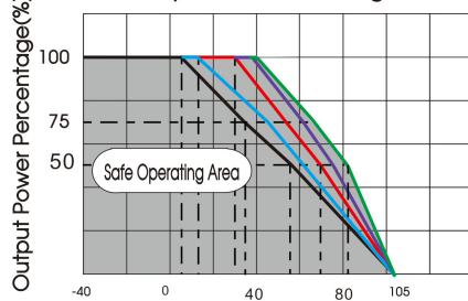
URF1D05QB-100WR3 temperature derating curve (Vin=110V)
