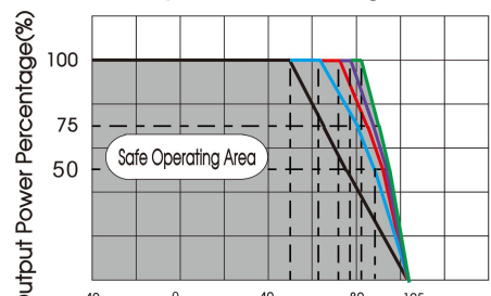
URF1D12QB-100WR3 temperature derating curve (Vin=110V)
