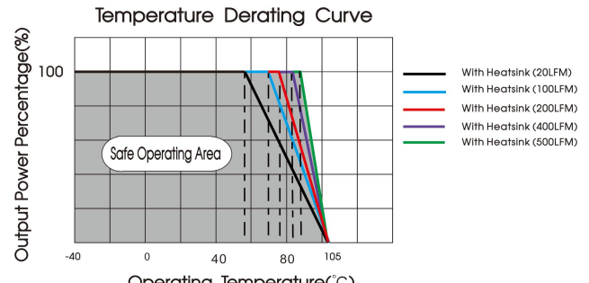
URF1D05QB-75WHR3 temperature derating curve (Vin=110V)
