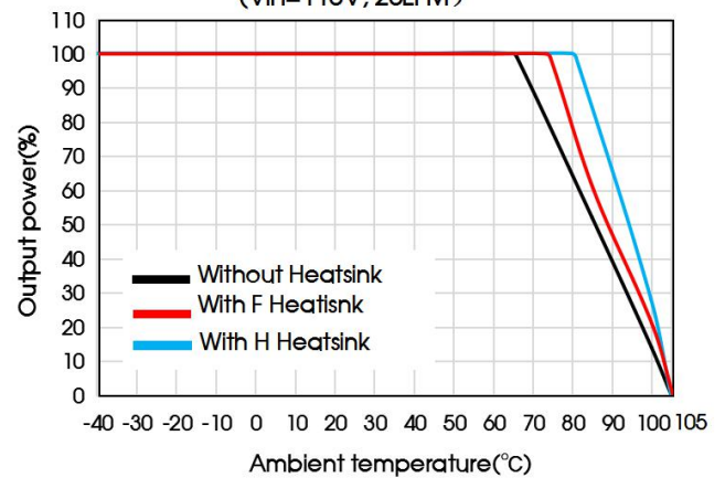
UWTH1D24/28/48/54QB-50WR3S Temperature Derating Curves ( V_{in}=110V , 20LFM)
