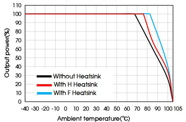
UWTH1D24/28/48/54QB-50WR3S Temperature Derating Curves (Vin=72V, 20LFM)
