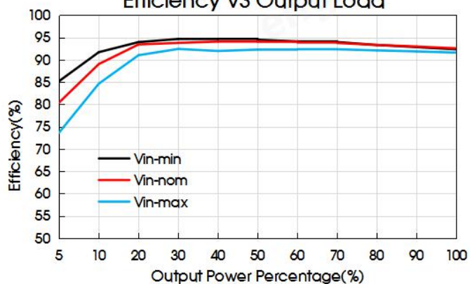
VRF2415HB-500WR3-N Efficiency VS Output Load
