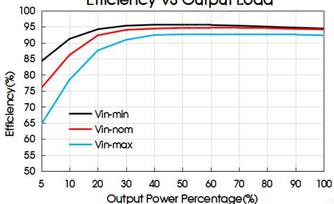
VRF2415HB-500WR3-N Efficiency VS Output Load
