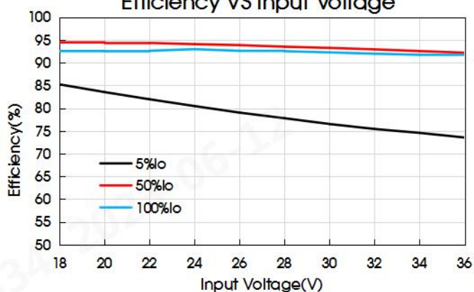
VRF2415HB-500WR3-N Efficiency VS Input Voltage
